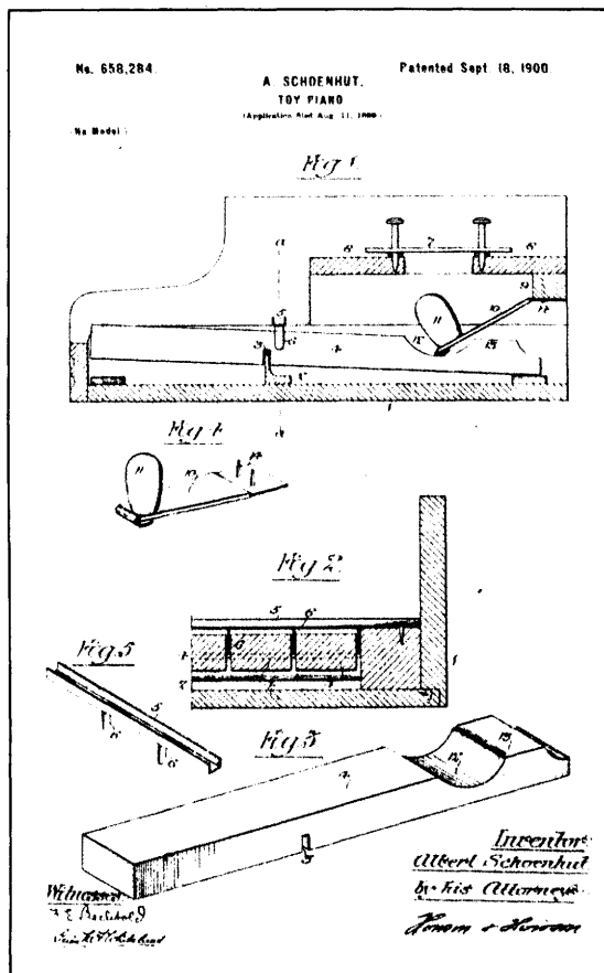
25. Patent drawing of toy piano mechanism invented by Albert Schoenhut
