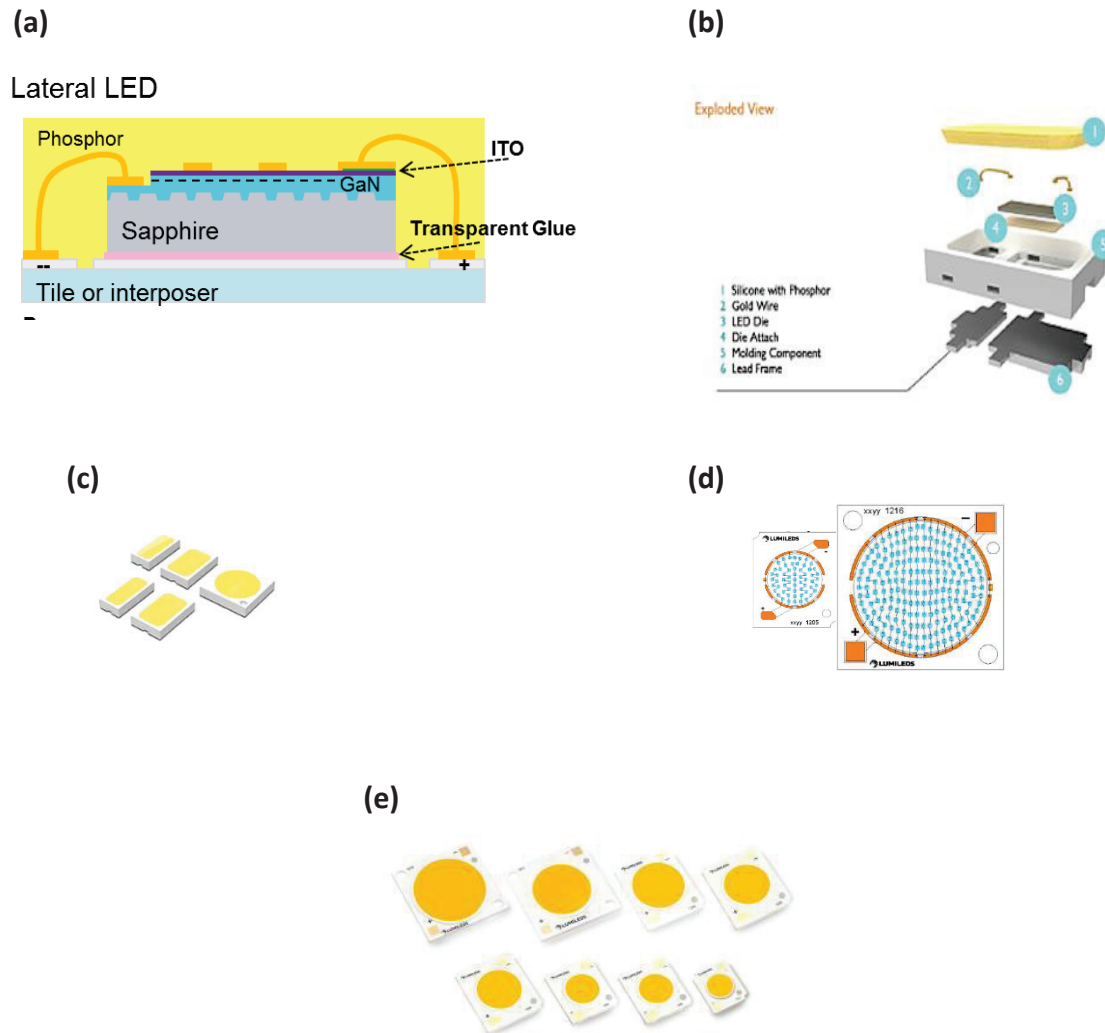
FIGURE 5.2 Lateral or edge-emitting package LED schematics. (a) mid-power (MP) or low-power (LP) light-emitting diode (LED) cross-section. The sapphire provides robust structure, and the low-cost package has the maximum extraction for non-directional applications. It is non-ideal for directional applications and has poorer heat sinking due to the use of transparent glue. The wire bond complicates phosphor integration; (b) MP/LP package schematic; (c) packaged MP/LP LED of varying sizes; (d) COB (chip-on-board) showing lateral die arrays; and (e) completed COB. NOTE: ITO = indium tin oxide. SOURCE: (a), (d), and (e) Courtesy of Lumileds; (b) and (c) Philips LSI Product Catalog, 2013 Version 1.0.
