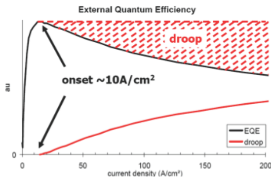
FIGURE 3.4 Schematic of light-emitting diode efficiency droop with increasing current density. The y-axis is a measure of external quantum efficiency (EQE), in arbitrary units (au). SOURCE: Denbaars, Speck, Nakamura, “Future Directions in SSL,” presentation to the committee, January 6, 2016. Courtesy University of California, Santa Barbara.
