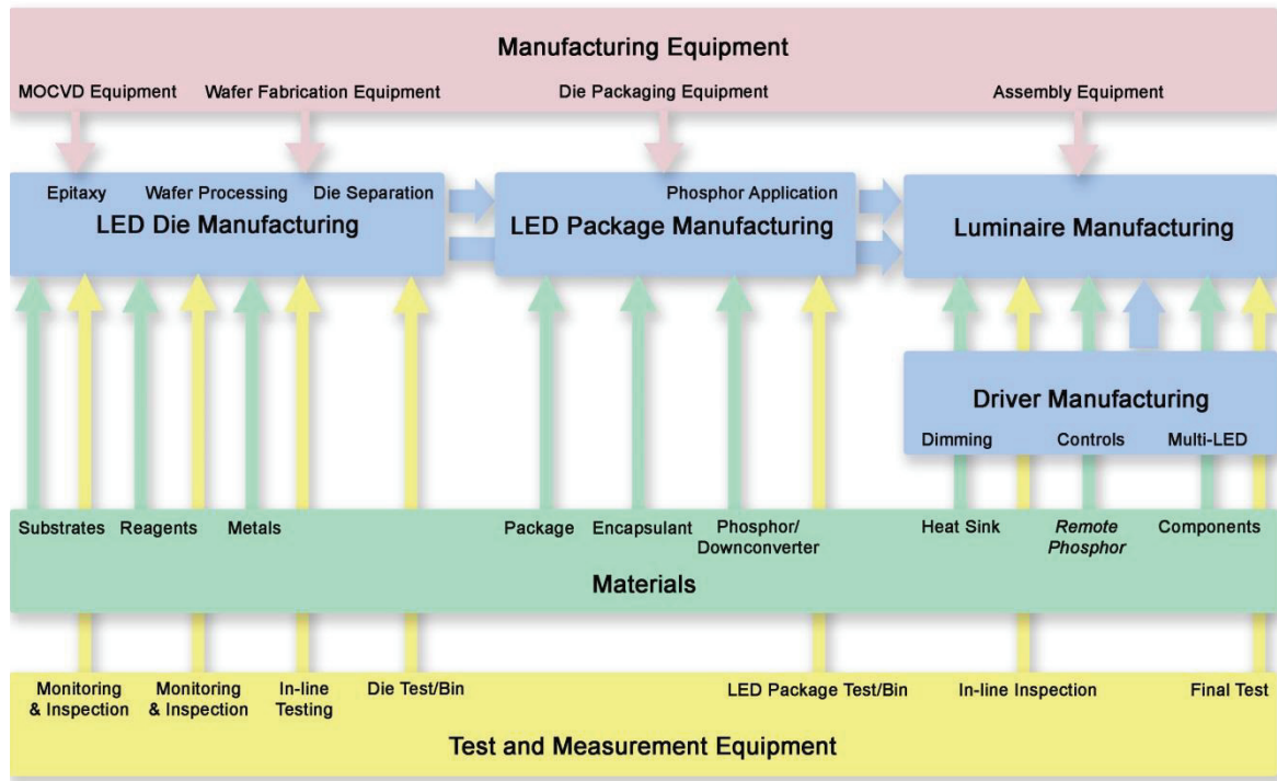
FIGURE 5.1 Light-emitting diode (LED)-based manufacturing supply chain. SOURCE: DOE (2015).
