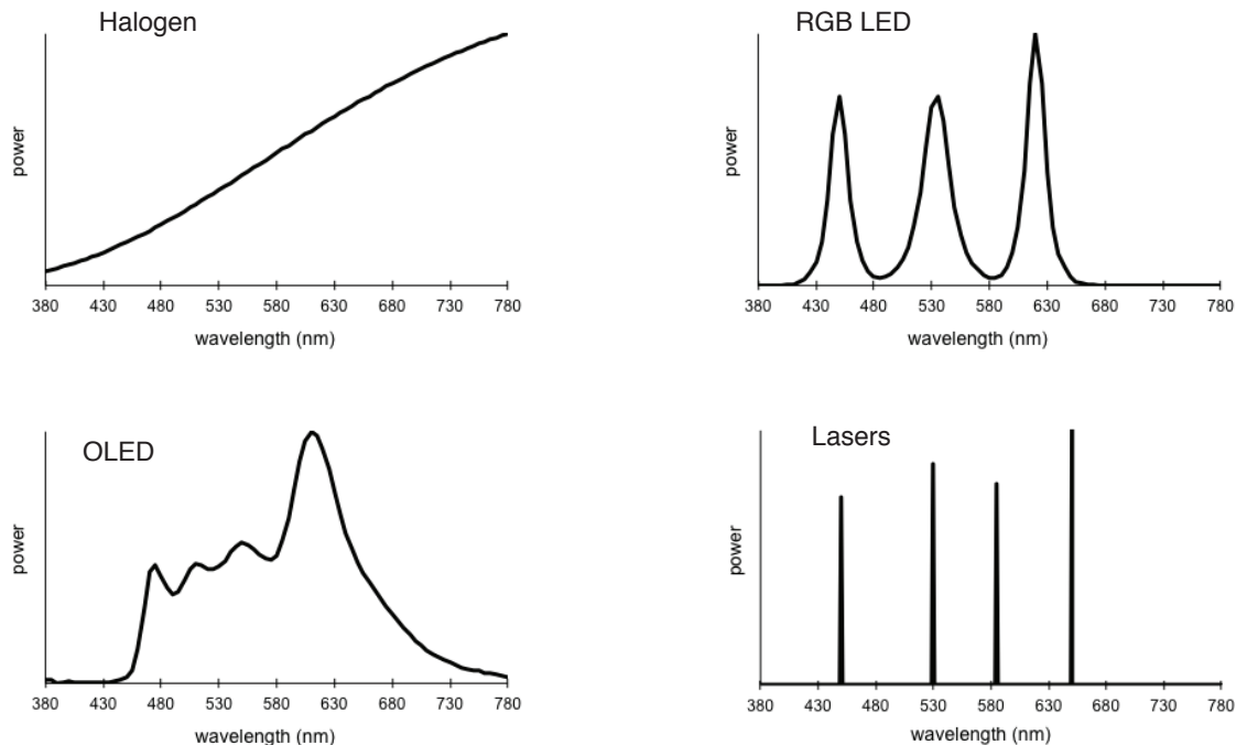
FIGURE C.7 Spectral power distribution from very different light sources that were chosen to produce identically appearing white light. The red, green, blue (RGB) light-emitting diode (LED) produces white light by combining red, green, and blue component LEDs, as does a combination of four colored lasers.
