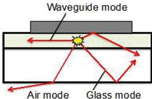
FIGURE 3.B.2 Illustration of the optical pathways taken by a photon following emission from a luminescent molecule (shown as yellow star).
