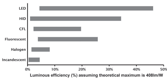
FIGURE C.6 Overall efficiencies of lighting systems (lower bounds) and devices (upper bounds) when assuming that the theoretical maximum lamp efficacy is 408 lm/W. NOTE: CFL = compact fluorescent lamp; HID = high-intensity discharge lamp; LED = light-emitting diode. Lower and upper bounds correspond to the low and high efficacy values shown in Figure C.5. © 2009 IEEE. Reprinted, with permission, from I.L. Azevedo, M.G. Morgan, and F. Morgan, 2009, The transition to solid state lighting. Proceedings of the IEEE 97:481-510.
