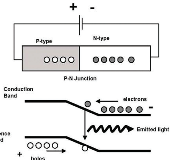
FIGURE 3.A.1 Schematic of p-n junction diode.
