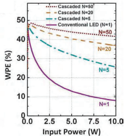
FIGURE 3.6 (a) Schematic of multiple p-n junctions, connected by tunnel junctions, (b) simulations showing the wall plug efficiency (WPE) of the light-emitting diode (LED), as a function of input power. SOURCE: Reprinted from F. Akyol, S. Krishnamoorthy, and S. Rajan, Tunneling-based carrier regeneration in cascaded GaN light emitting diodes to overcome efficiency droop, Applied Physics Letters 103(8):1107, with the permission of AIP Publishing.
