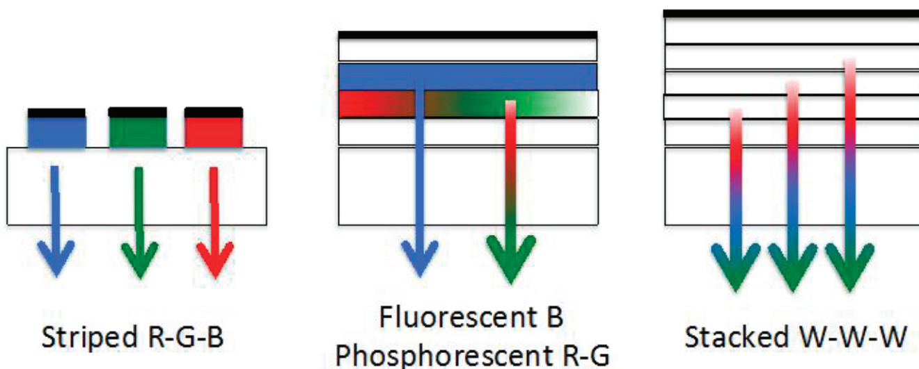
FIGURE 3.B.3 Three examples of white organic light-emitting diode designs.
