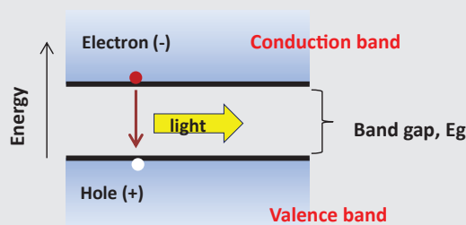
FIGURE 3.A.1.1 Light emission process.
