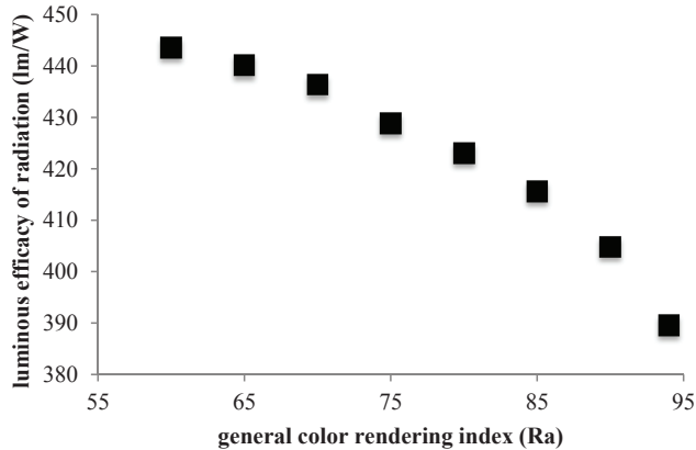
FIGURE 1.2 Maximum luminous efficacy of radiation as a function of general color rendering index ( R_a ) for spectral power distribution consisting of four wavelengths of spectral power, with correlated color temperature = 3,000 K and Duv = 0.000 .
