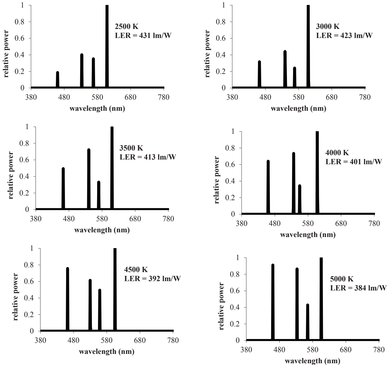
FIGURE 1.1 Maximum luminous efficacy of radiation (LER) for spectral power distributions (SPDs) consisting of four wavelengths of spectral power at six different correlated color temperatures. For all SPDs, Duv = 0.000 and color rendering index ( R_a ) = 80.
