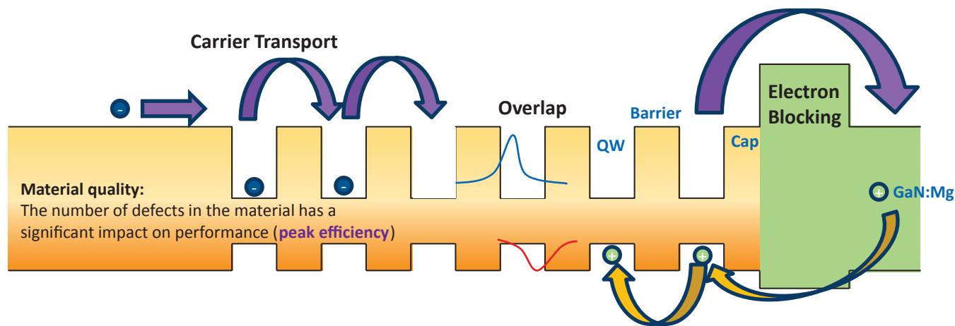
FIGURE 3.A.2 Schematic of a multiple quantum well (QW) region, showing injection of electrons (in purple, from left) and holes (in yellow, from right). The desired goal is recombination of electrons and holes to form photons. The schematic suggests the ways in which electrons and holes may be lost from the structure or otherwise not be able to recombine. SOURCE: Image courtesy Lumileds, Epitaxy Technology Group.
