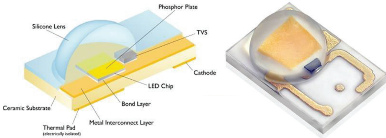
FIGURE 3.A.4 Schematic of a light-emitting diode (LED) module. SOURCE: Lumileds.
