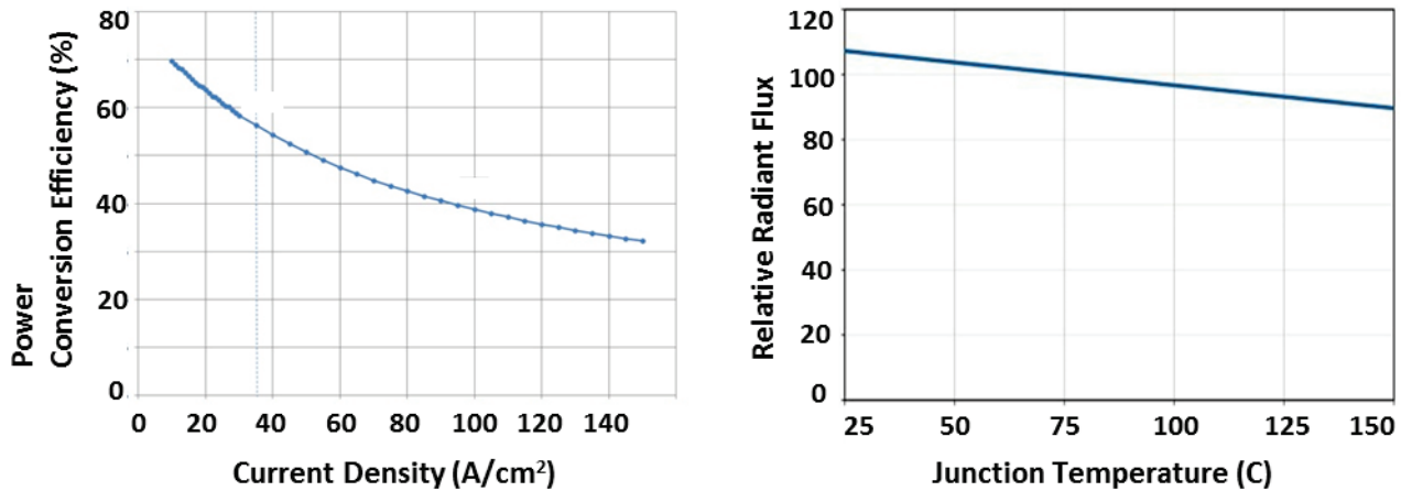
FIGURE 3.2 Two types of efficiency droop: (a) current efficiency droop and (b) thermal efficiency droop. SOURCE: Cree XLamp XT-E Datasheet.
