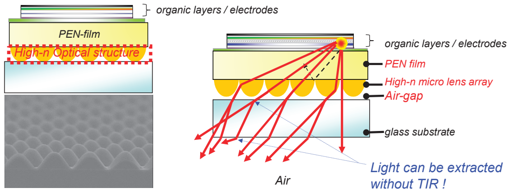
FIGURE 3.13 Light extraction scheme for a Panasonic panel, using (left) high-index substrate and (right) high-index microstructure; both external. SOURCE: K. Yamae, H. Tsuji, V. Kittichungchit, N. Ide, and T. Komoda, 2013, High-performance white-OLED devices for next-generation solid-state lighting, SID Information Display 29(5):38-44, September/October. ©2014 Society for Information Display.
