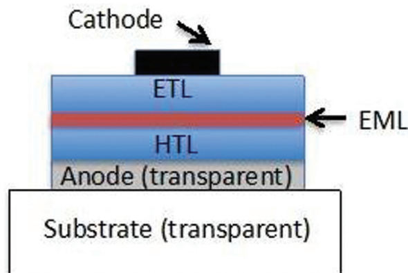
FIGURE 3.B.1 Archetype organic light-emitting diode structure. SOURCE: A.E. Willner, R.L. Byer, C.J. Chang-Hasnain, S.R. Forrest, H. Kressel, H. Kogelnik, G.J. Tearney, C.H. Townes, and M.N. Zervas, 2012, Optics and photonics: Key enabling technologies, Proceedings of the IEEE 100:1604. ©IEEE (2012). Reprinted, with permission from Proceedings of the IEEE.
