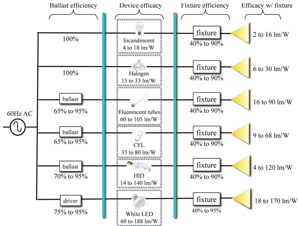
FIGURE C.5 Efficacy of lamps and luminaires. Values in the left-most column report the range of efficiencies for ballasts and electronic drivers. Values in the central column report efficacies for different lighting devices. The values on the third column report ranges of luminaire efficiencies. The values on the right-most column report the overall system efficacies of the luminaire. Figure adapted from Azevedo et al. (2009), where the efficacies for white LEDs were updated to reflect currently commercialized warm and cool white LEDs. © 2009 IEEE. Reprinted, with permission, from I.L. Azevedo, M.G. Morgan, and F. Morgan, 2009, The transition to solid state lighting. Proceedings of the IEEE 97:481-510.
