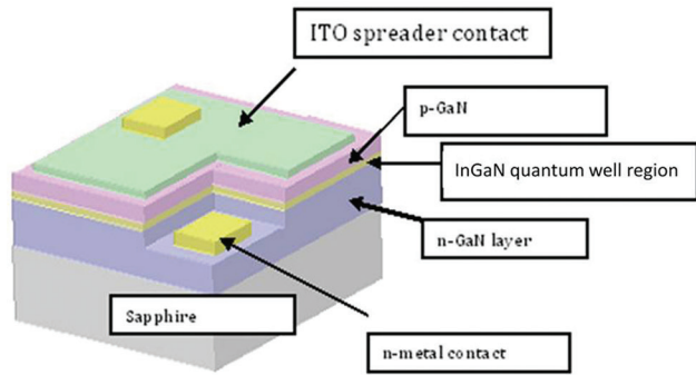
FIGURE 3.A.3 A typical GaN light-emitting diode (LED) chip.
