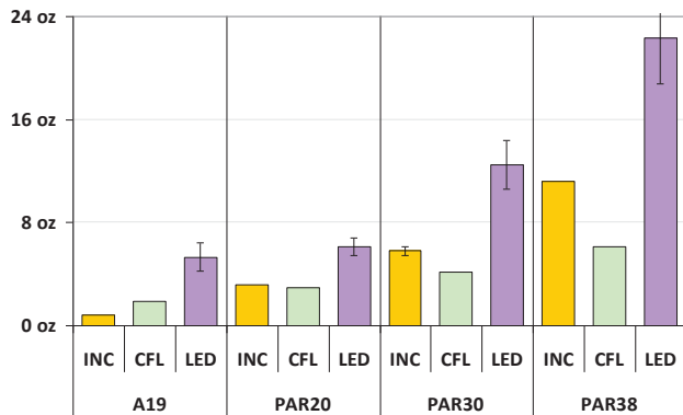
FIGURE 4.A.1 Weight comparisons among incandescent (INC), compact fluorescent (CFL), and LED lamps for A19, PAR20, PAR30, and PAR38 lamp types. SOURCE: N. Narendran, Y. Gu, J.P. Freyssinier-Nova, and Y. Zhu. 2005. Extracting phosphor-scattered photons to improve white LED efficiency. Physica Status Solidi A 202(6):R60-R62.
