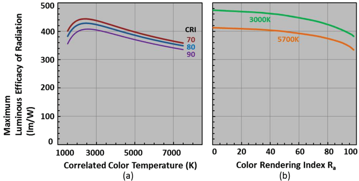
FIGURE 3.3 Theoretical limits to white light luminous efficacies versus (a) correlated color temperature (CCT) for a given color rendering index (CRI) and (b) CRI for a given CCT. SOURCE: DOE (2016). Courtesy Jeffrey Tsao, Sandia National Laboratories.
