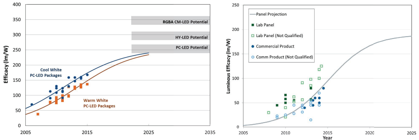
FIGURE 3.1 (a) Efficacies of commercial light-emitting diode (LED) packages measured at 25°C and 35 amperes per square meter ( A/cm^2 ) input current. Blue data points and fit for “cool white” lighting (5,700 K); orange data points and fit for “warm white” lighting (3,000 K). Gray bars indicate approximate long-term, future potential efficacies for three white-light architectures: phosphor-coated LEDs (pc-LEDs), “hybrid” technology LEDs (hy-LEDs), red, blue, green, and amber (RGBA) color-mixed LEDs (cm-LEDs). (b) White-light organic light-emitting diode panel efficacy projections. SOURCE: DOE (2016).
