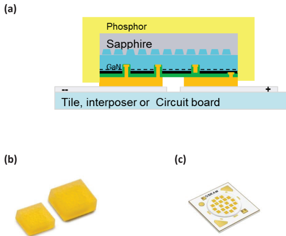
FIGURE 5.5 Chip scale package (CSP). (a) Cross-section of CSP. The contact/heat sinking does not interfere with light emission, and the sapphire provides robust structure for direct attachment; (b) 1 mm and 2 mm CSP parts for direct attachment; and (c) CSP-based arrays on boards—similar to chip-on-board, but with higher output. SOURCE: (a and b) Lumileds; (c) Osram GmbH.
