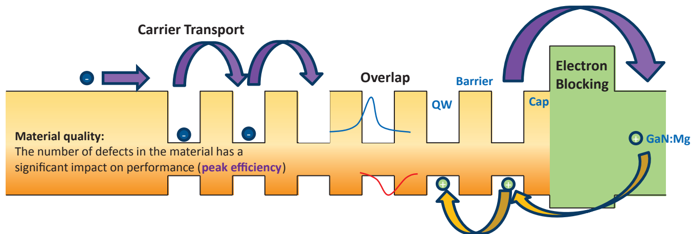
FIGURE 3.5 Schematic of a multiple quantum well (QW) region, showing injection of electrons (in purple, from left) and holes (in yellow, from right). The desired goal is recombination of electrons and holes to form photons. The schematic suggests the ways in which electrons and holes may be lost from the structure or otherwise not be able to recombine. SOURCE: Image courtesy Lumileds, Epitaxy Technology Group.
