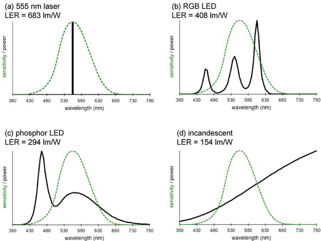
FIGURE C.9 Spectral power distribution determines luminous efficacy of radiation (LER). The dashed green curves show the Spectral Luminous Efficiency Function, and the black curves are light source’s spectral power distributions. NOTE: RGB = red, green, blue.
