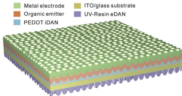
FIGURE 3.15 Schematic showing both internal and external scattering layers produced by soft-lithographic nano-imprinting. SOURCE: Q.-D. Ou, L. Zhou, Y.-Q. Li, S. Shen, J.-D. Chen, C. Li, Q.-K. Wang, S.-T. Lee, and J.-X. Tang, 2014, Extremely efficient white organic light-emitting diodes for general lighting, Advanced Functional Materials 24(46):7249-7256. © 2014 WILEY-VCH Verlag GmbH & Co. KGaA, Weinheim.
