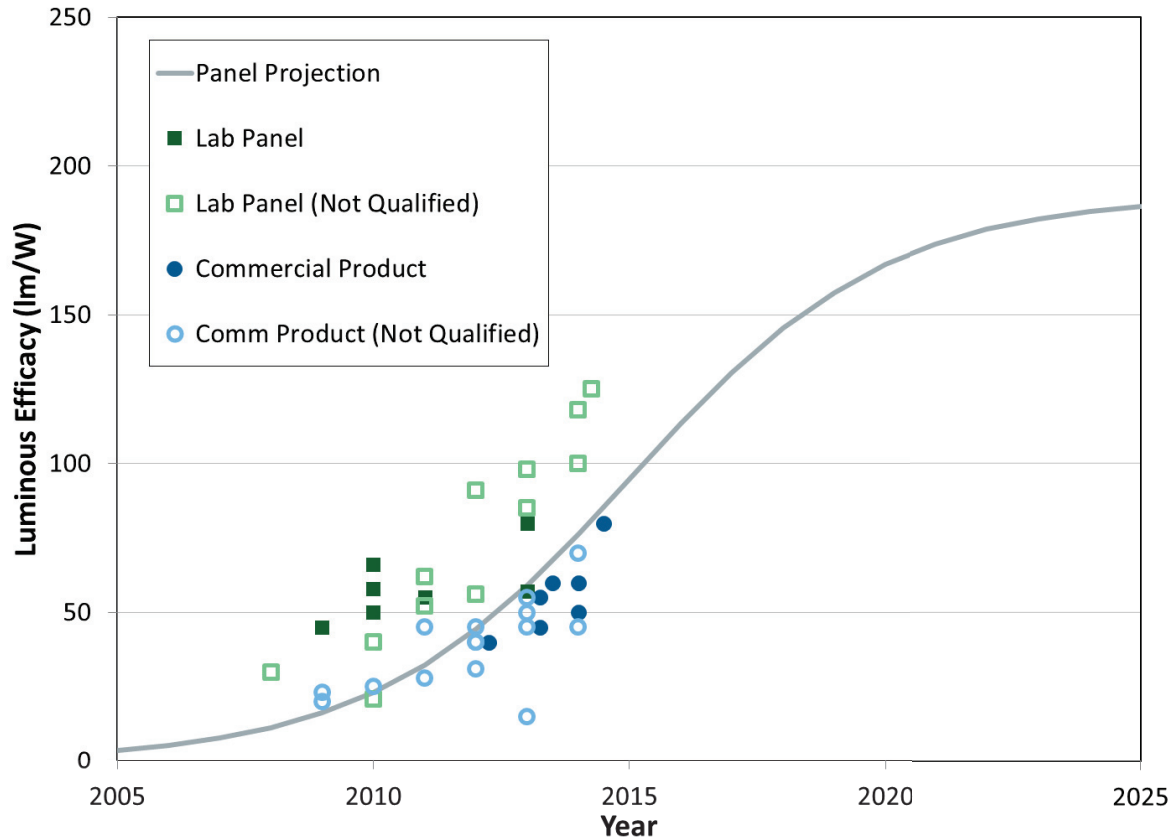
FIGURE 3.10 Projection of organic light-emitting diode efficacy. SOURCE: DOE (2016, p. 139).
