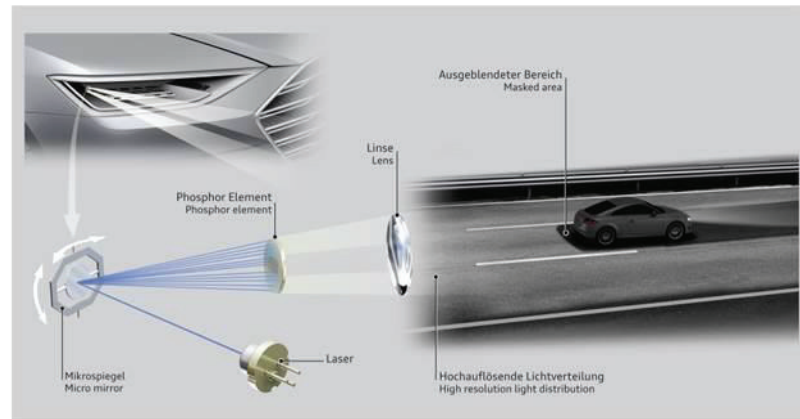
FIGURE 4.3 Audi's Matrix laser headlights. SOURCE: L. Ulrich, 2015, Audi pixelated laser headlights light the road and paint it too, IEEE Spectrum , May 6, http://spectrum.ieee.org/cars-that-think/transportation/advanced-cars/audi-lights-the-road-with-pixelated-laser-headlights .
