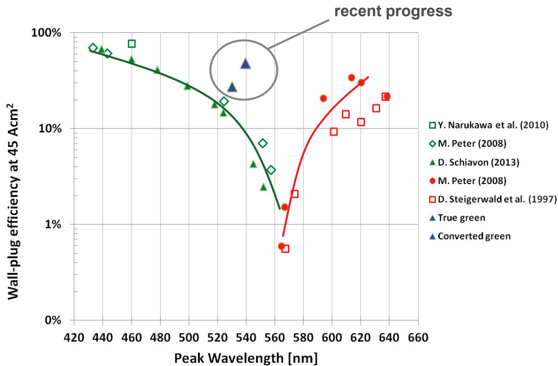
FIGURE 3.8 Light-emitting diode wall plug efficiency as a function of wavelength. Note that the axis of wall plug efficiency is given on a logarithmic scale. SOURCE: B. Hahn, OSRAM, “Closing the Green Efficiency Gap,” presentation at DOE Solid-State Lighting R&D Workshop, Raleigh, N.C., February 3, 2016. Courtesy OSRAM GmbH.
