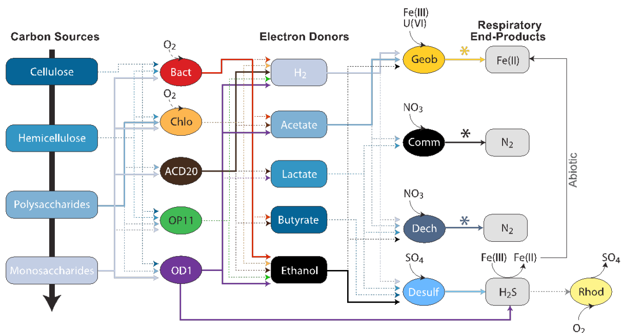
Figure 2-2 Uncultivated candidate phyla (brown, green, purple ovals) contain a wide variety of carbohydrate active enzymes that drive respiratory metabolisms linked to the cycling of hydrogen, metals, and sulfur. Predicted metabolic and geochemical interactions are supported by genomic (dashed lines) and proteomic (solid lines) analyses. The fermentation of carbon results in the production of organic acids and hydrogen by a phylogenetically novel fermentative community including candidate phyla lineages (OD1, OP11, ACD20), and uncultivated members of Chloroflexi and Bacteroidetes. These fermentation metabolites can fuel iron, sulfur, and nitrogen cycles driven by members of the Proteobacteria, including well-known uranium-reducing bacteria such as Geobacter .
