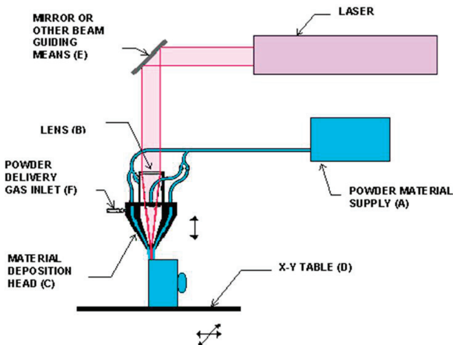
FIGURE 7.15 Laser Engineered Net Shaping (LENS TM ) process schematic. SOURCE: Worldwide Guide to Rapid Prototyping Website, © Copyright Castle Island Co., all rights reserved. Available at http://www.additive3d.com/len_int.htm . Reprinted with permission.
